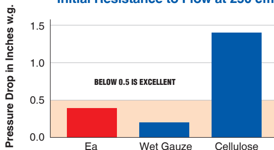
Initial Resistance to Flow at 250 cfm
